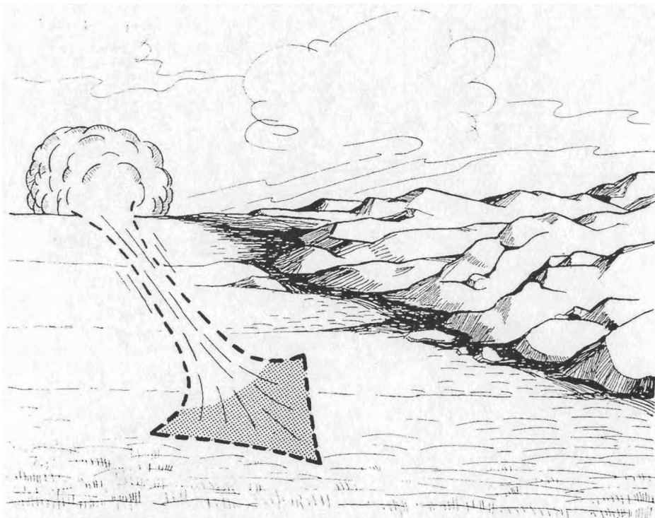
Figure 34. Effect of wind on open terrain.
