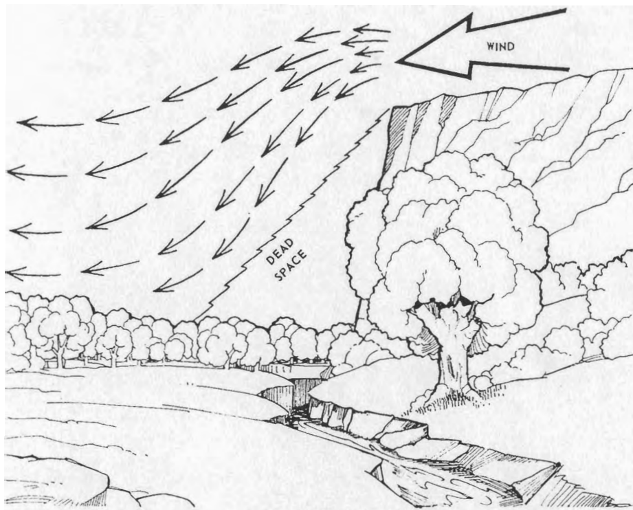
Figure 36. Effect of wind blowing from a mesa.
